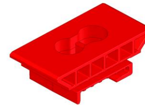
Description Bearing H32 pos.point, 2 hole 6,5 mm (red) with vertical lip Art. no. 4107018
